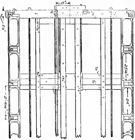
Fig. 360. Port Plan of Underframe.
